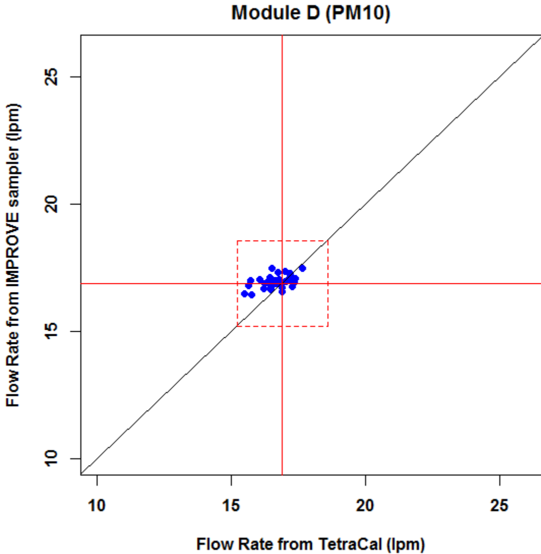
Figure 5. Flow rate comparisons for Module D audits in 2017.
