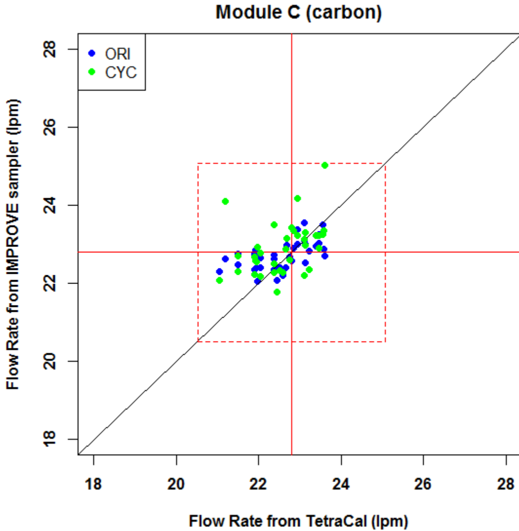
Figure 4. Flow rate comparisons for Module C audits in 2017.
